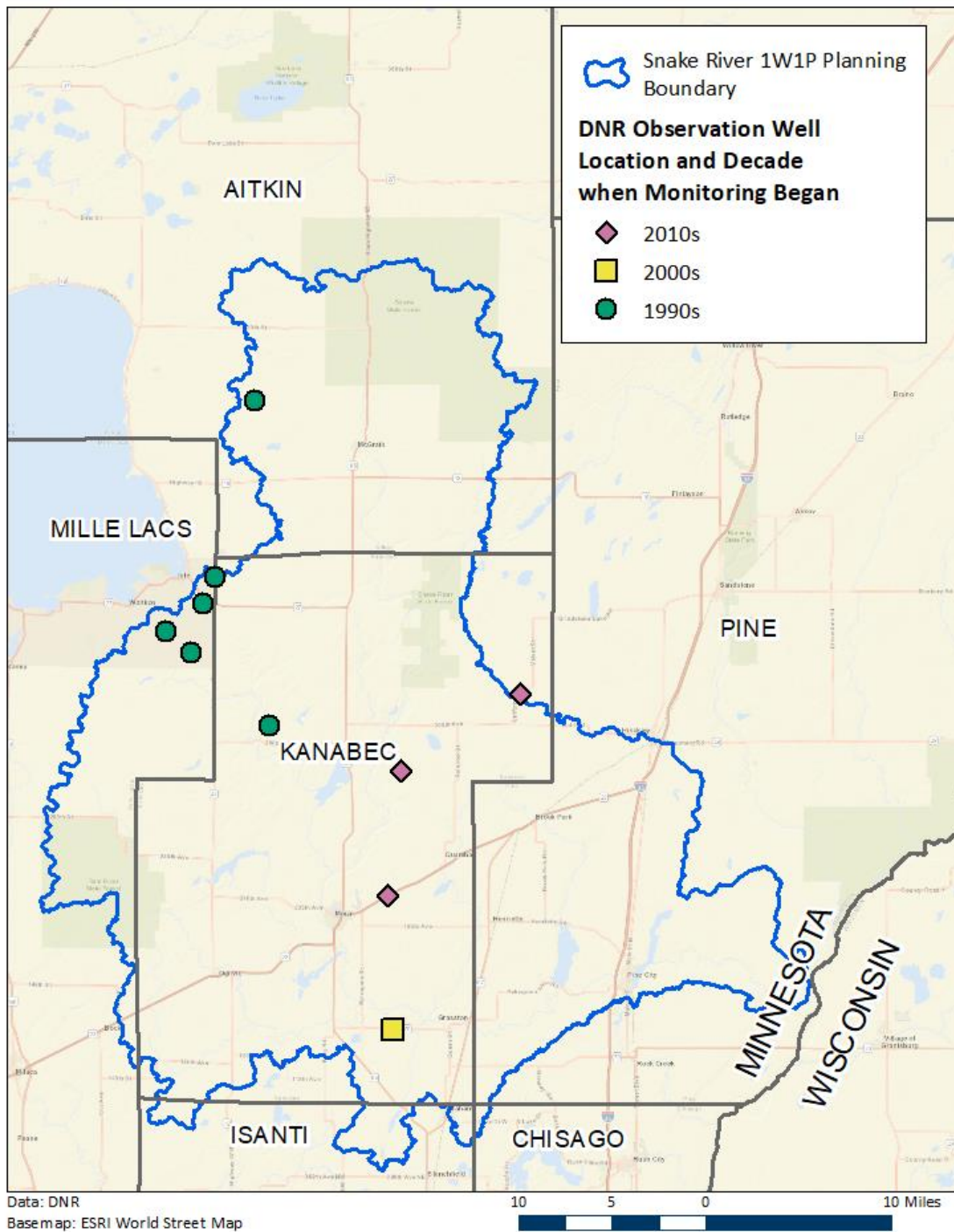
Figure 25: Snake River Watershed – Active Groundwater-Level Monitoring Wells in the Snake Watershed by decade monitoring started. Six of the groundwater-level monitoring wells in the watershed have been monitored since the 1990s. One monitoring well was added in the 2000s and three wells were added in the 2010s.
